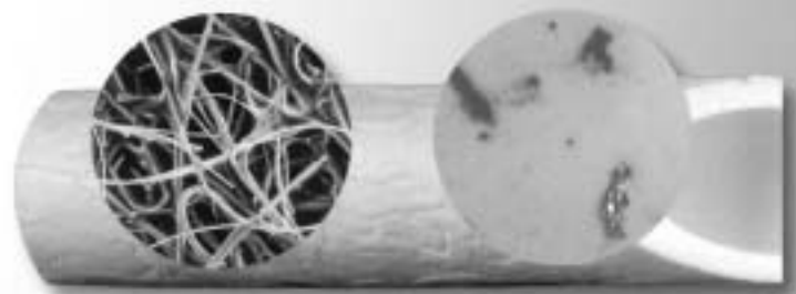
Scanning electron micrograph (at 228x)
